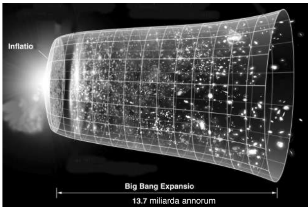
Expansio Universi, qualis nunc fingitur (Wikipedia)
