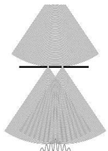
Experimentum Thomæ Young (Wikimedia).
