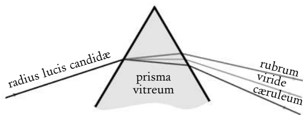
Refractio lucis radii prisma transeuntis
