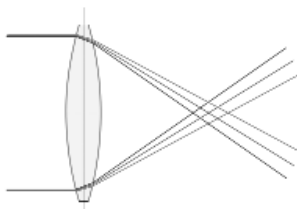
Aberratio chromatica (Wikimedia)
