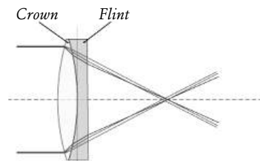
Correctio aberrationis chromatiæ (Wikimedia)
